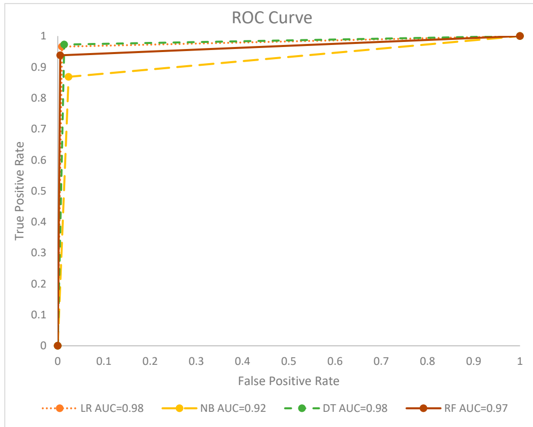
Figure 5. The ROC curve results (all classifiers).
