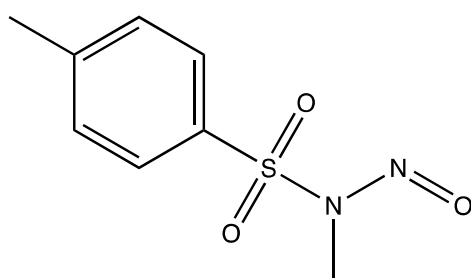
Scheme 4. N-methyl-N-nitroso-p-toluenesulfonamide (MNTS).
