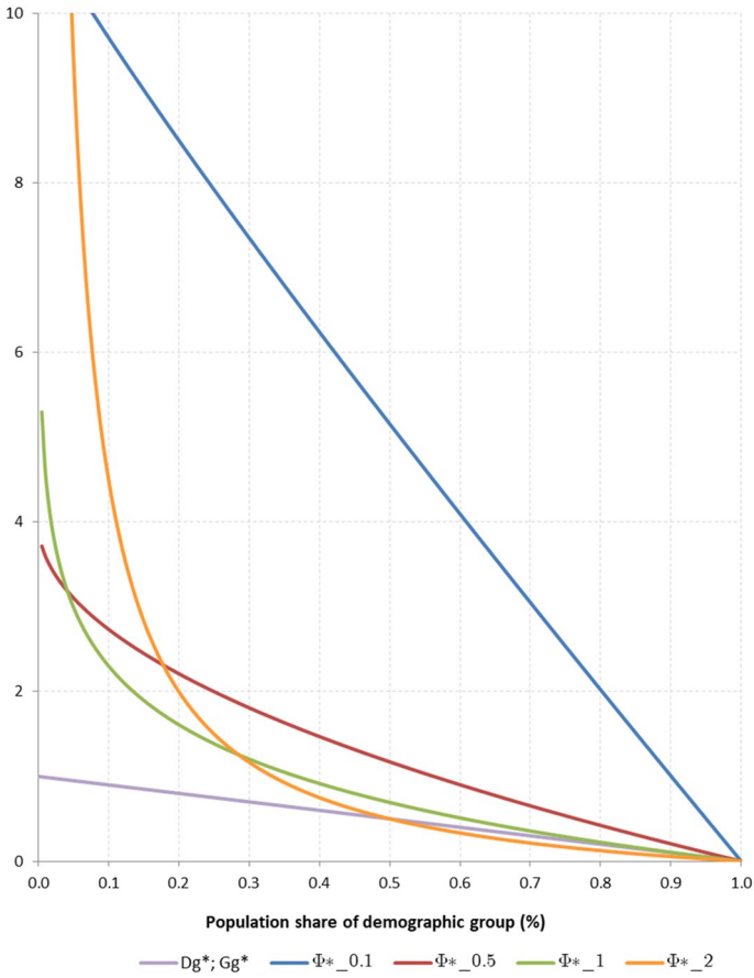
Fig. 7 Maximum local segregation ( D^{g^*} , G^{g^*} , \Phi_{0.1}^{g^*} , \Phi_{0.5}^{g^*} , \Phi_1^{g^*} , and \Phi_2^{g^*} )
