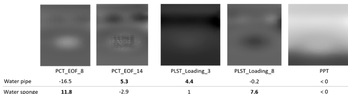
Figure 3. Best SNR results (black numbers) regarding the detection of the water recirculation through the pipe and the water propagation from the sponge, applying PCT, PLST and PPT and following experiment 2 of reference [3]. A description of the methodology here applied can be found in [4].
