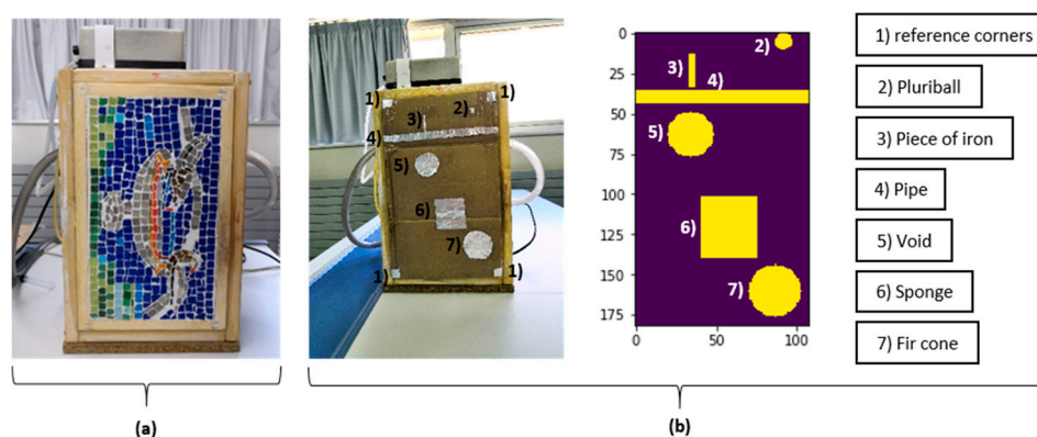
Figure 1. (a) Mosaic to be tested, seen from its front surface; (b) Frontal representation of the situation of each of the artificial internal defects.
